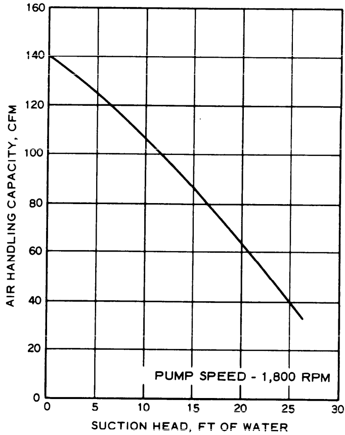
Figure 4-32. Characteristics of typical vacuum unit for wellpoint pumps.
