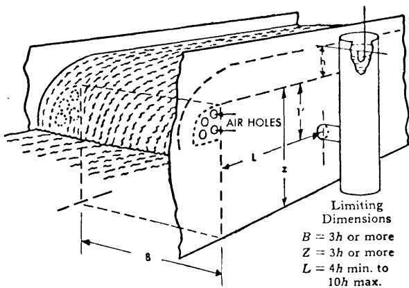
Figure F-9. Rectangular suppressed weir.
