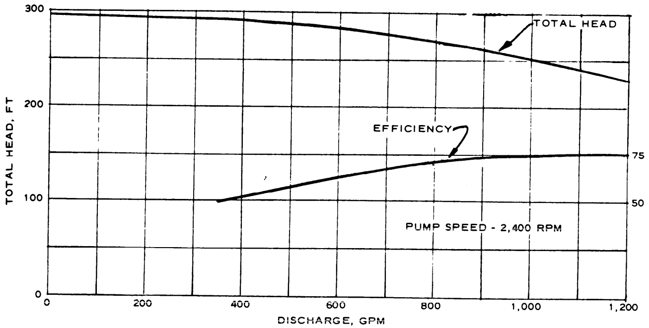
Figure 4-33. Characteristics of 6-inch jet pump.
