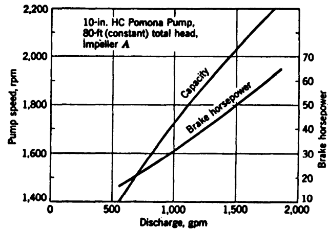
Figure 4-35. Rating curves for a three-stage 10-inch-high capacity deep-well pump.
