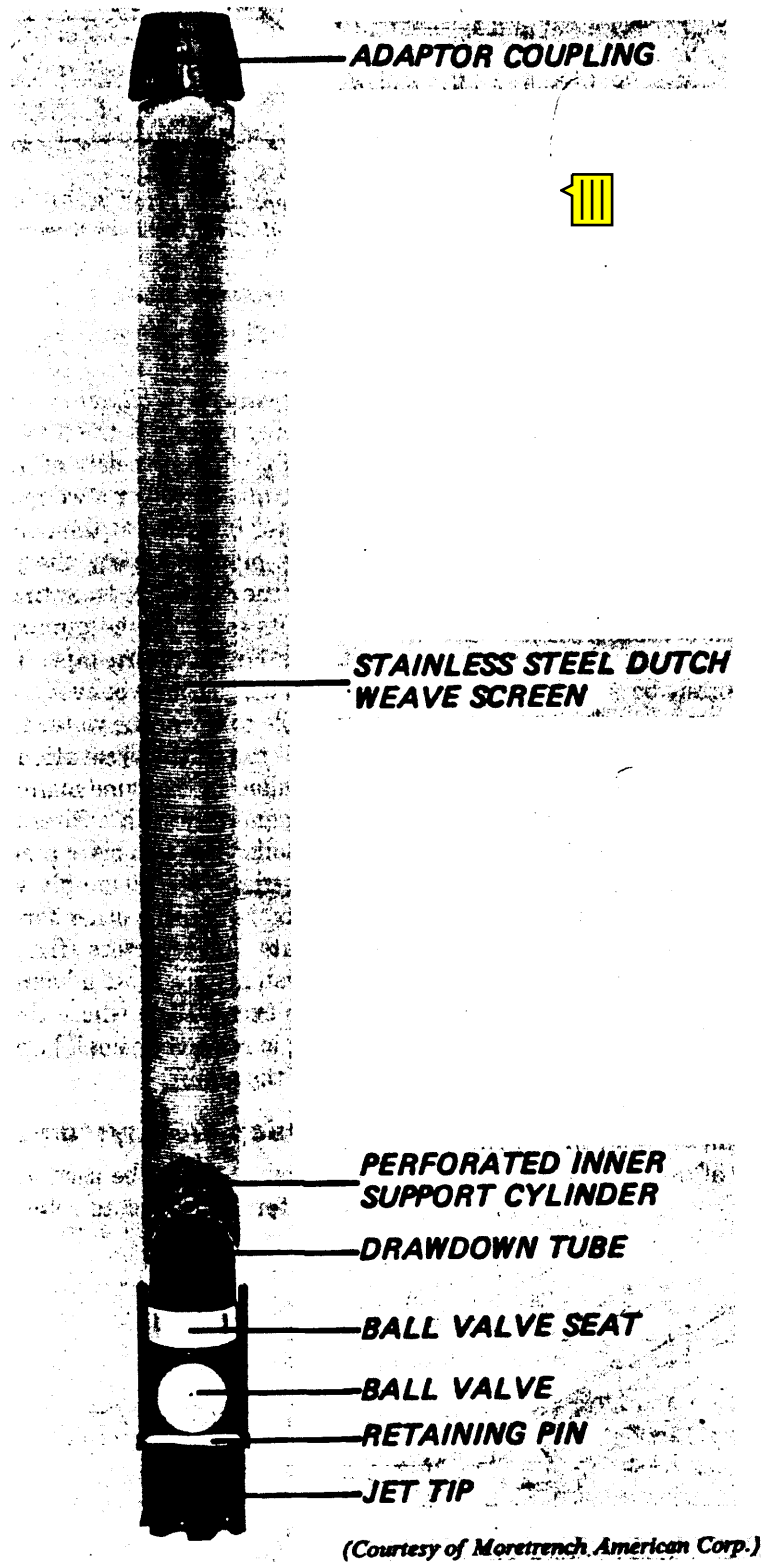
Figure 2-2. Self-jetting wellpoint.
